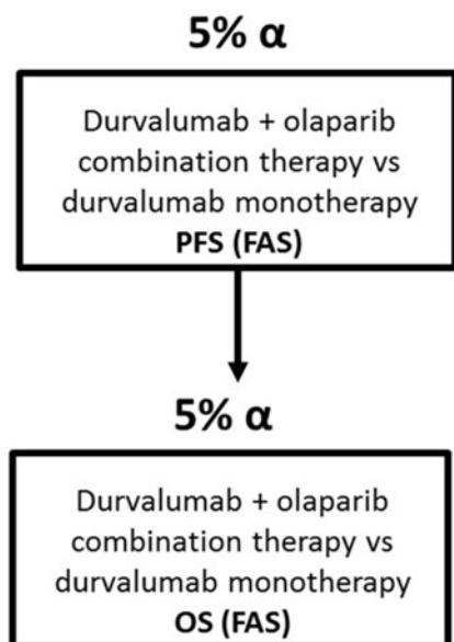
Figure 2 Multiple Testing Procedure
